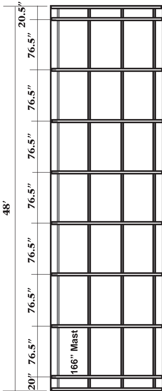
HF Mast Spacing 14' x 48'
