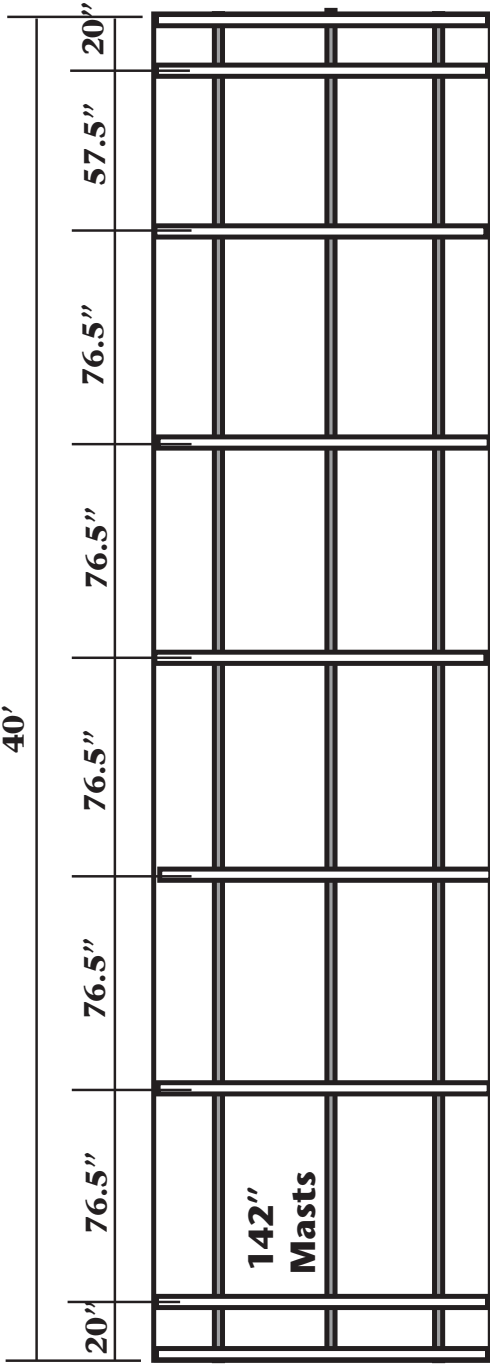
HF Mast Spacing 12' x 40'
