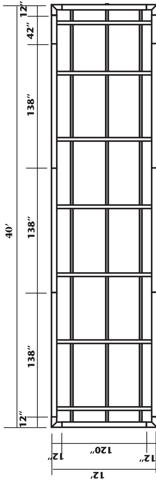
HF Frame Spacing 12' x 40'
