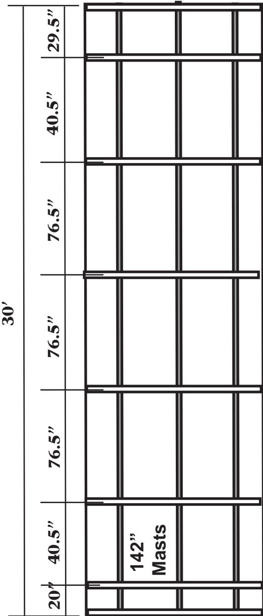
HF Mast Spacing 12' x 30'
