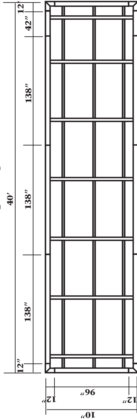
HF Frame Spacing 10' x 40'
