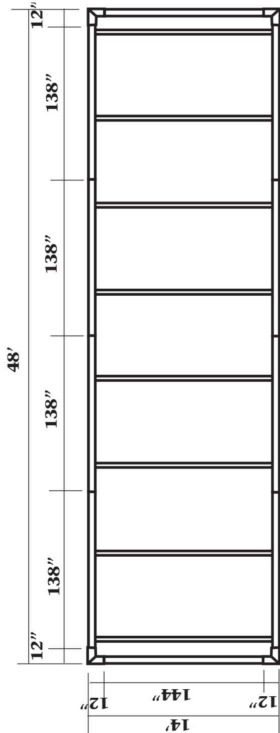
HF Frame Spacing 14' x 48'
